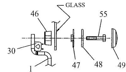
TYPICAL THROUGH GLASS BOLTING PATTERN. 4X SCALE
