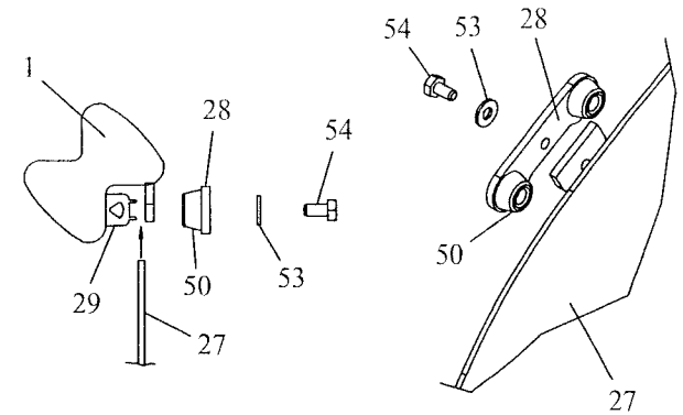
WINDOW CLAMP INSTALL 4X SCALE
